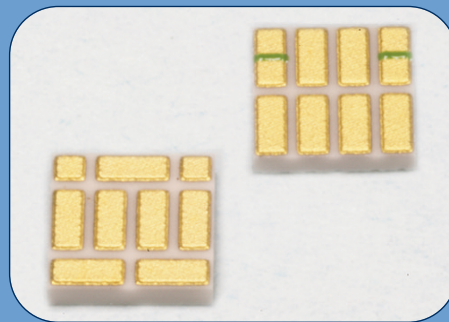
Substrate for a miniature TEC cooler. Use of AgENIG metallization with .0025" thick silver deposits and 0.35 mΩ/sq resistivity allowed current carrying capacity in excess of 10 AMP.
