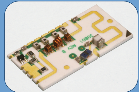
Substrate for a miniature TEC cooler. Use of AgENIG metallization with .0025" thick silver deposits and 0.35 mΩ/sq resistivity allowed current carrying capacity in excess of 10 AMP.
