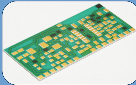
Substrate with AgENIG metallization, plated through-holes and printed resistors for a peak detector.
